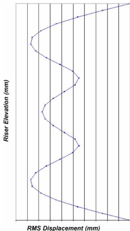
RMS Displacement Profile of Riser 5th May 1999 09:01 to 09:21
